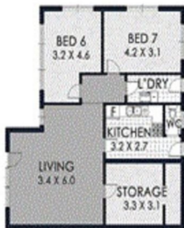
LOWER FLOOR
