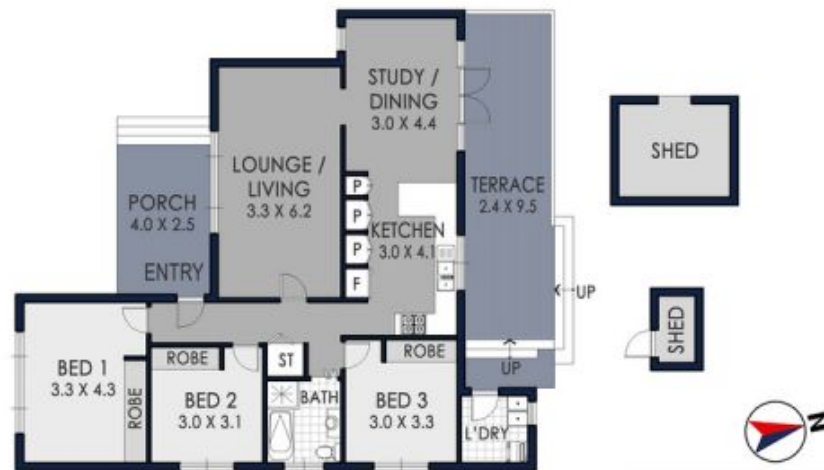
FLOOR PLAN
